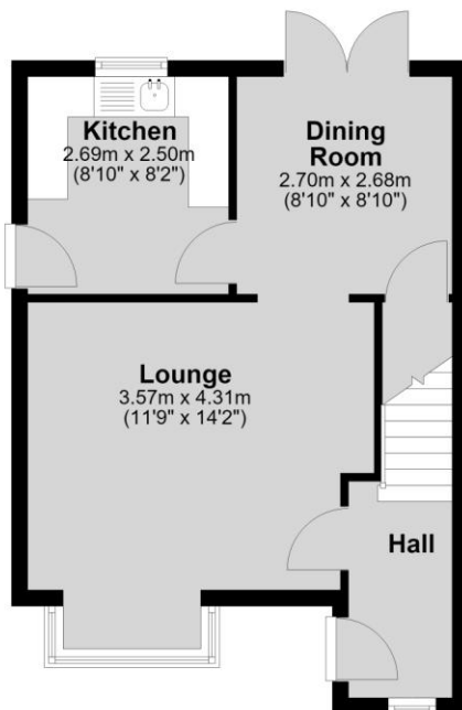
Ground Floor Approx. 36.0 sq. metres (387.0 sq. feet)
