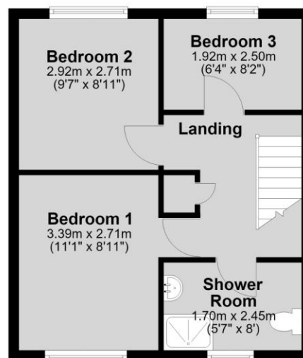
First Floor Approx. 34.9 sq. metres (375.5 sq. feet)
