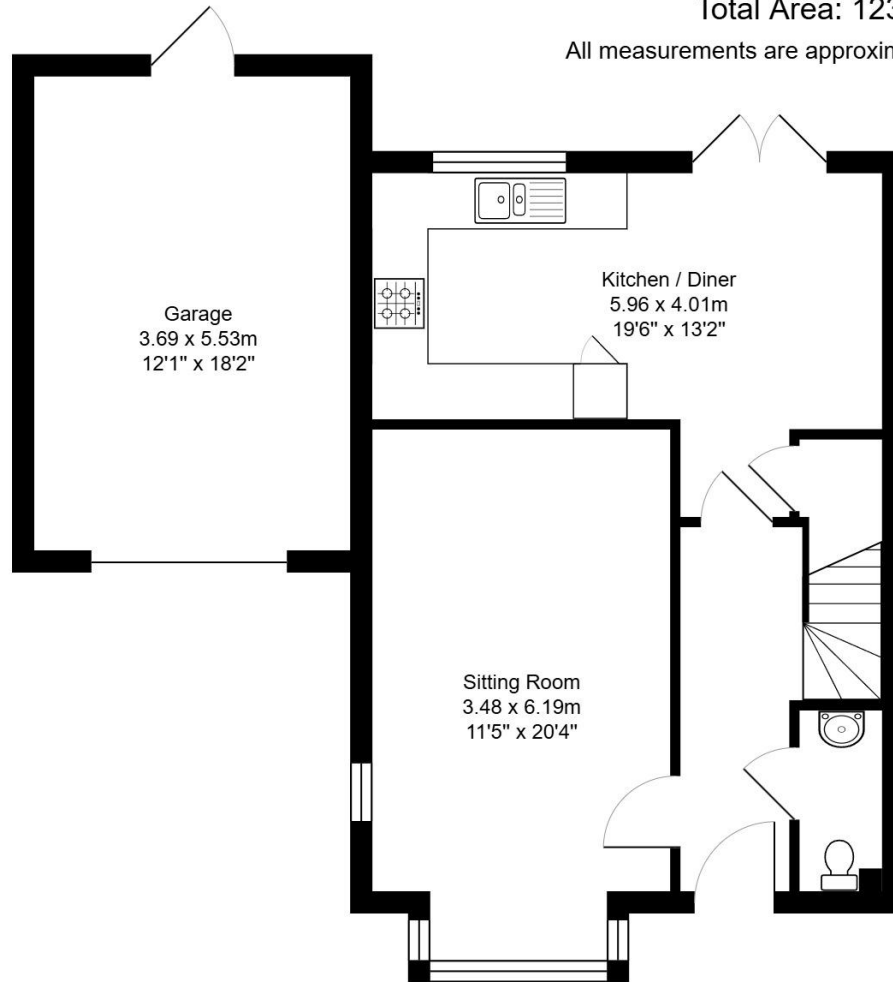
Ground Floor Area: 73.2 m 2 ... 787 ft 2
