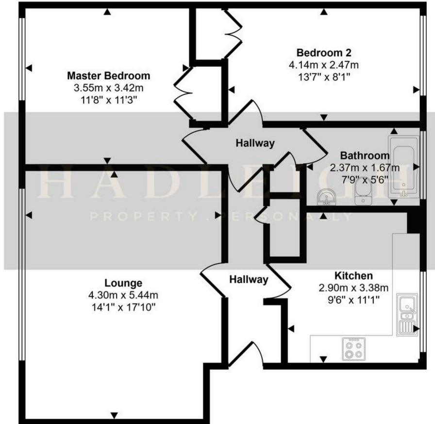
Floorplan
