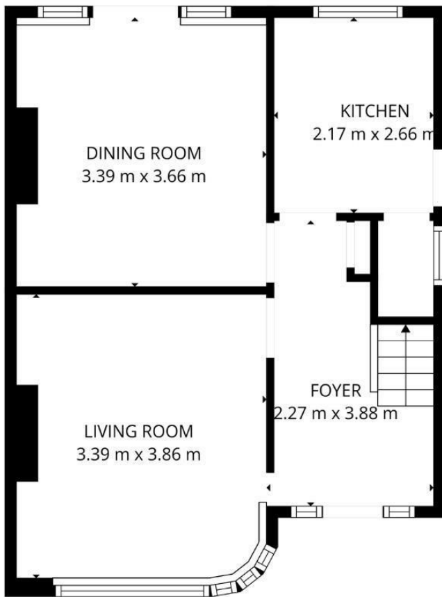
FLOOR 1
