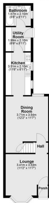
Ground Floor Approx. 44.8 sq. metres (481.7 sq. feet)
