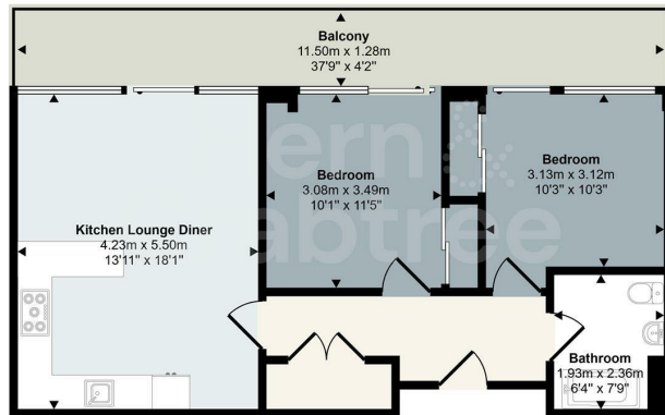
Floorplan
