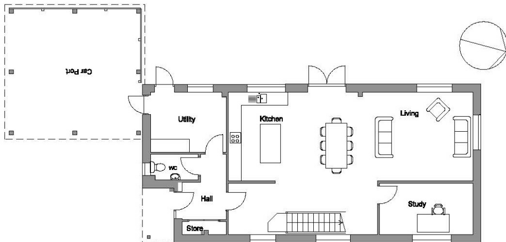
Plot 1 Ground floor plan
