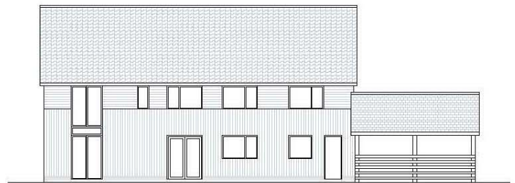
Plot 1 West elevation
