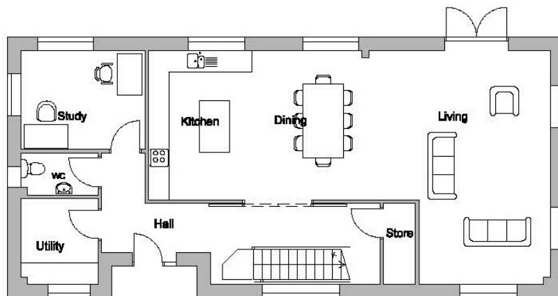
Plot 3 Ground floor plan
