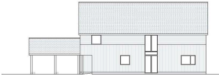
Plot 1 East elevation
