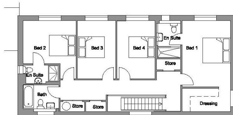
Plot 1 First floor plan
