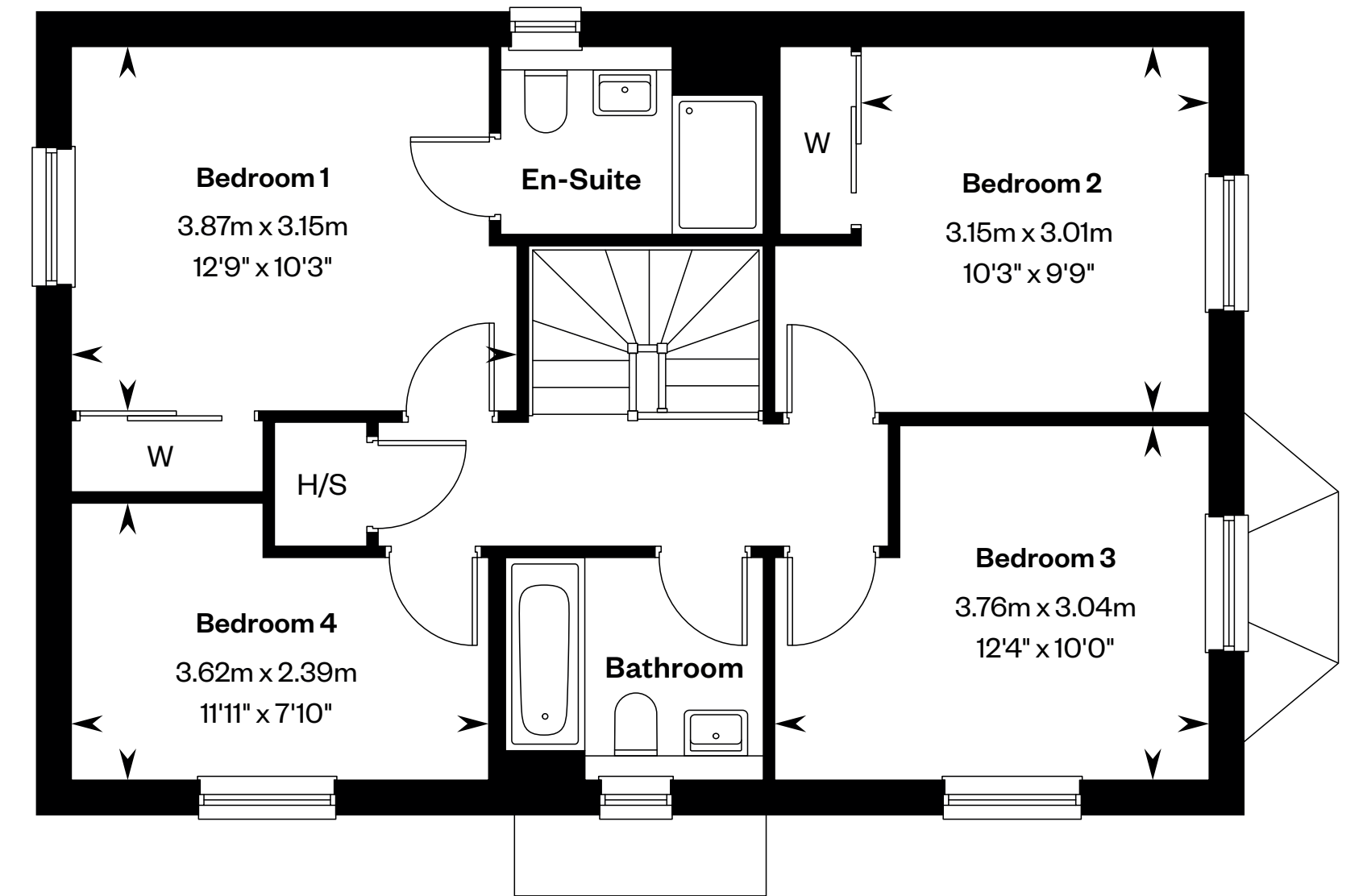
First floor
