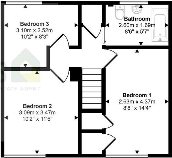
First Floor Approx 42 sq m / 457 sq ft
