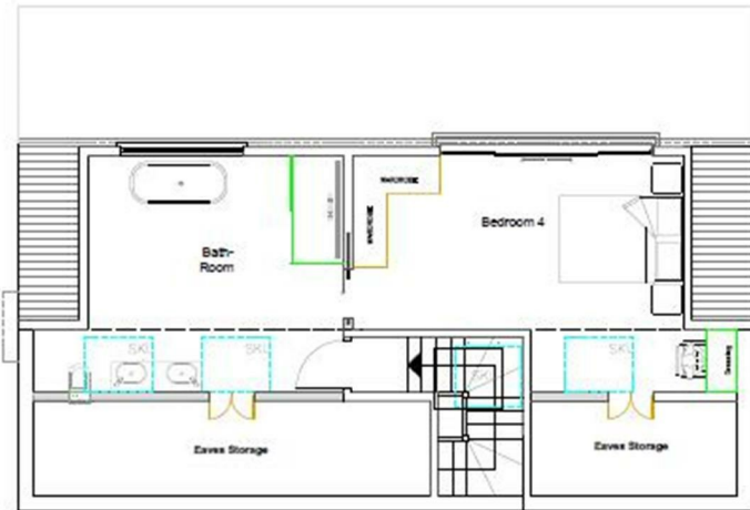
Proposed Second Floor Scale 1:100
