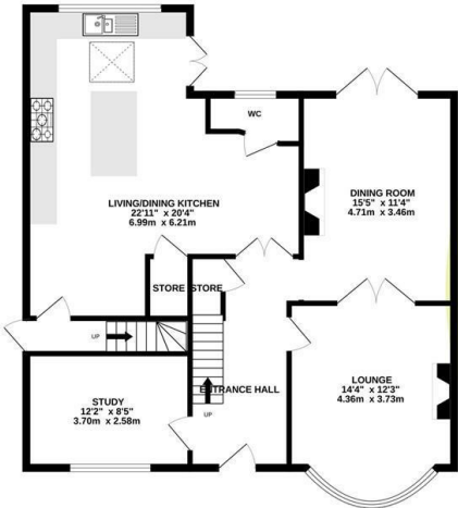
GROUND FLOOR 958 sq.ft. (89.0 sq.m.) approx.
