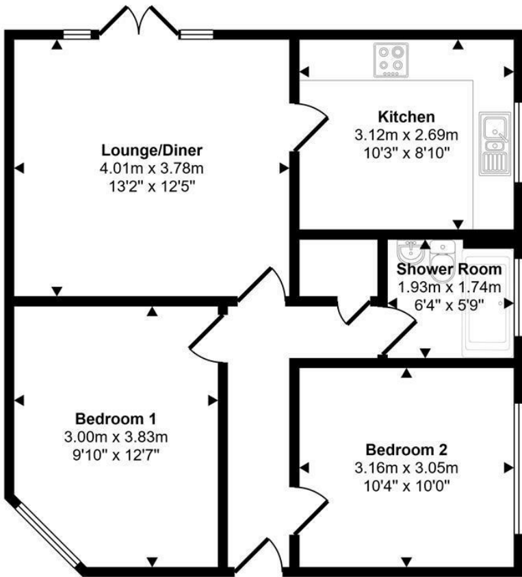
Floorplan
