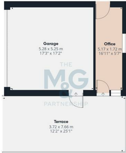
Floor 0 Building 2
