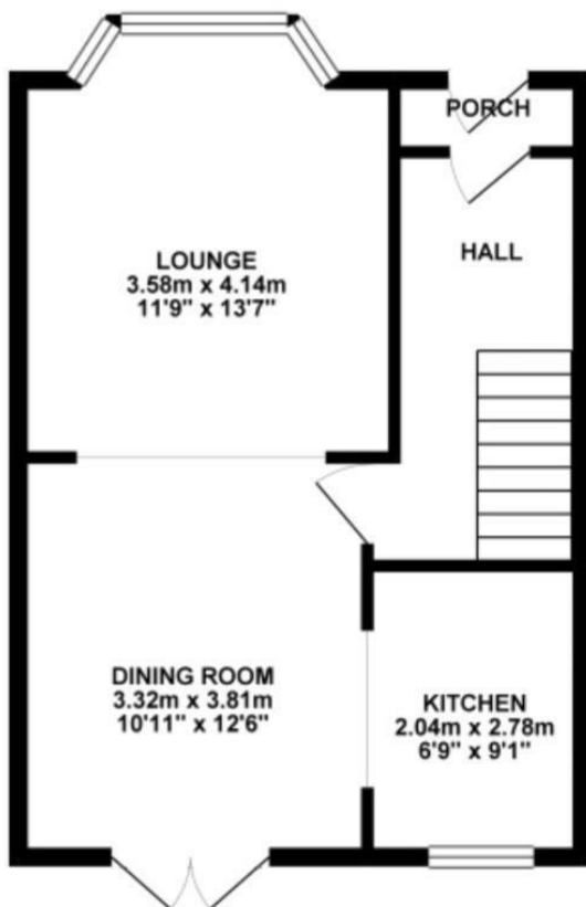
GROUND FLOOR 40.89 sq. m. ( 440.11 sq. ft. )
