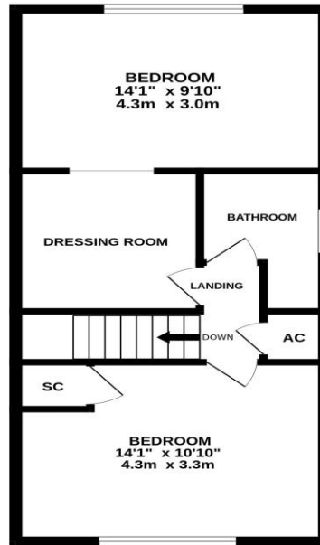
1ST FLOOR 457 sq.ft. (42.4 sq.m.) approx.
