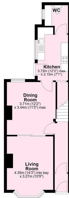
Ground Floor Approx. 43.7 sq. metres (470.4 sq. feet)
