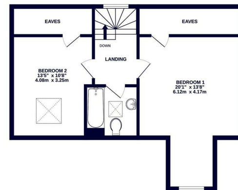
1ST FLOOR 557 sq.ft. (51.7 sq.m.) approx.
