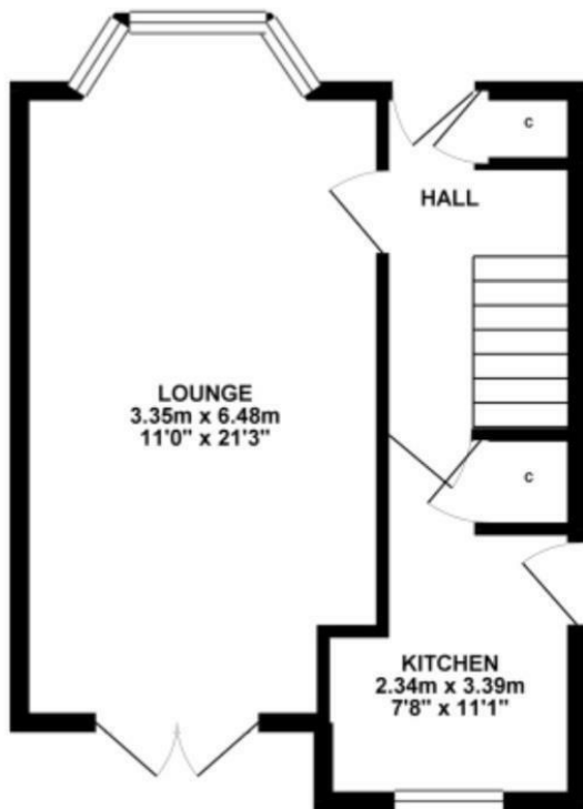
GROUND FLOOR 32.89 sq. m. ( 354.00 sq. ft. )
