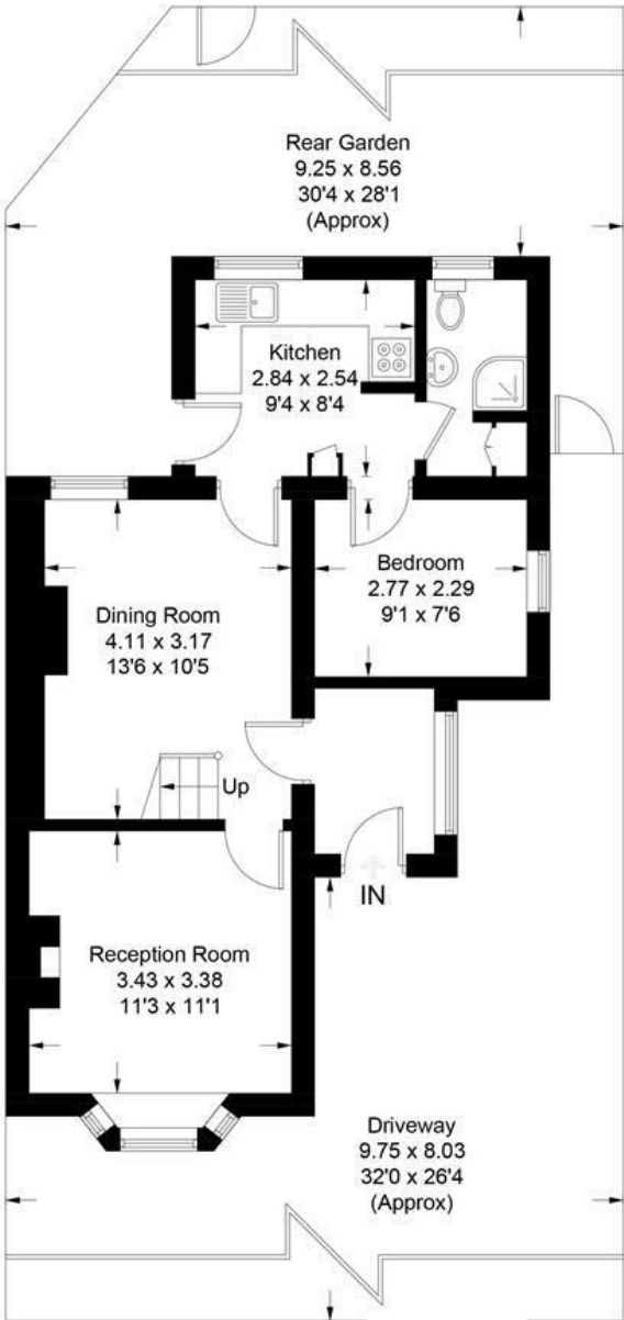
Ground Floor
