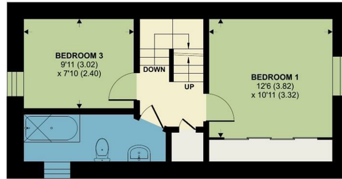
FIRST FLOOR
