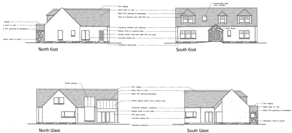
Plot 1 - Elevations
