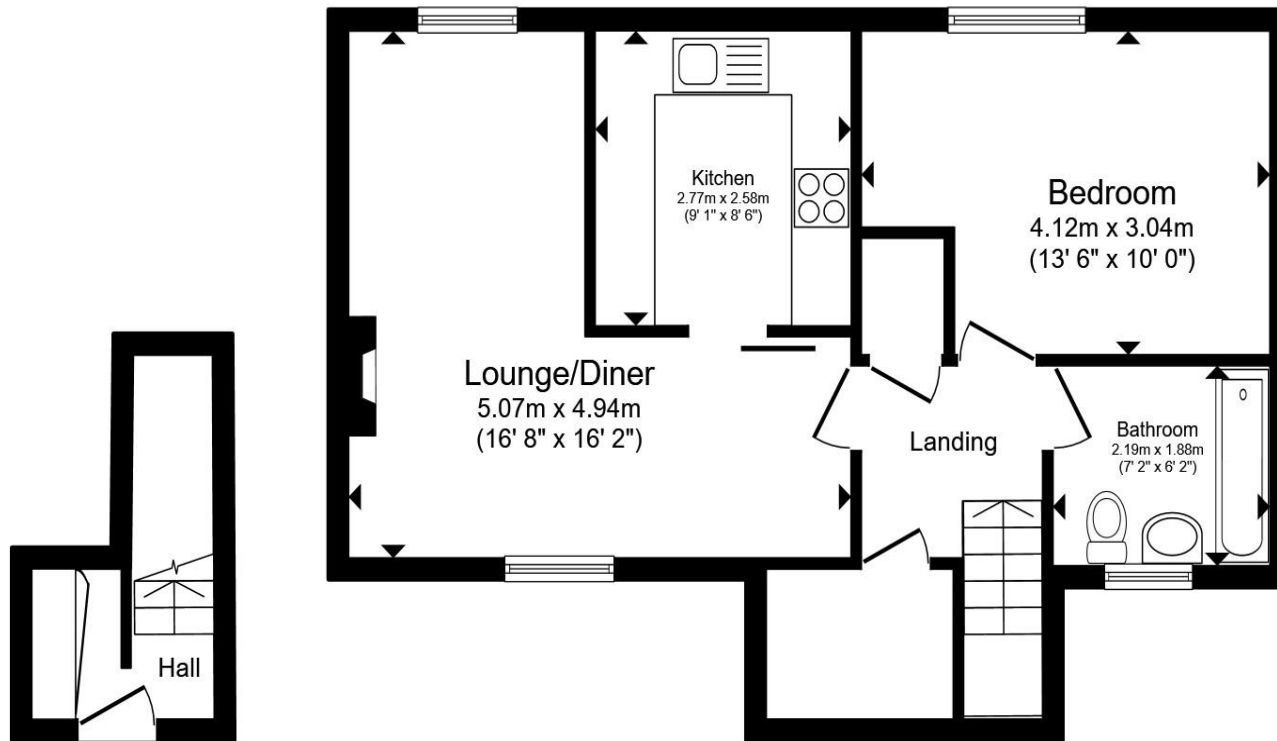
Ground Floor
