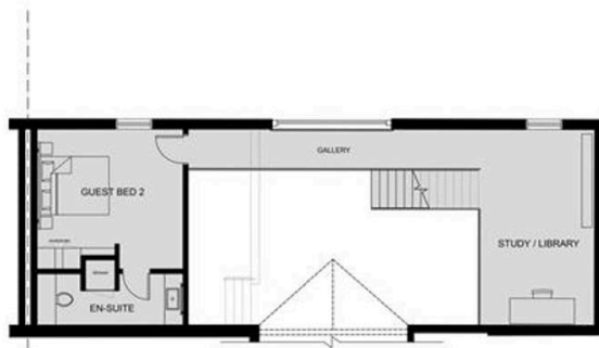
PROPOSED FIRST FLOOR (58.5Sqm / 630Sqft)
