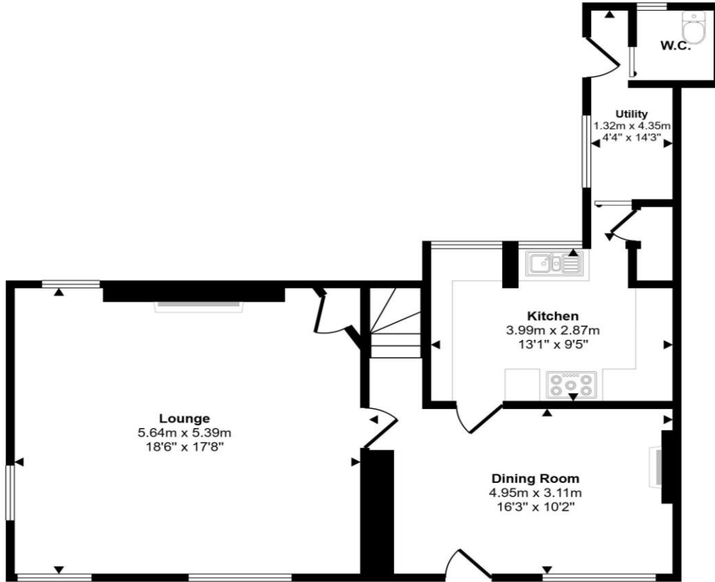
Ground Floor Approx 68 sq m / 728 sq ft
