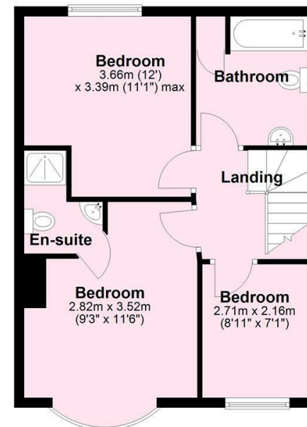
First Floor Approx. 46.02 SQ metres 495 SQ feet
