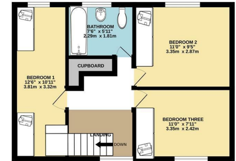
1ST FLOOR 392 sq.ft. (36.4 sq.m.) approx.
