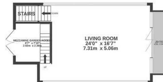
THIRD FLOOR
