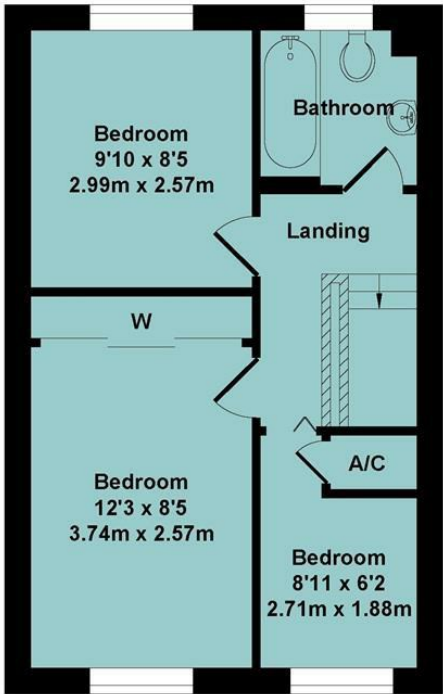
First Floor Approx. Floor Area 358 Sq.Ft. (33.30 Sq.M.)
