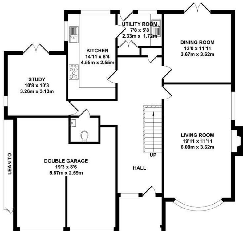
GROUND FLOOR APPROX. FLOOR AREA 1269 SQ.FT. (117.89 SQ.M.)
