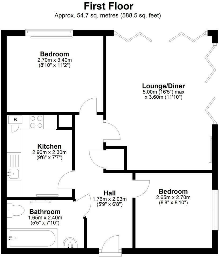
Total area: approx. 54.7 sq. metres (588.5 sq. feet)
