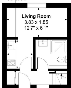
Ground Floor (Unit 3)
