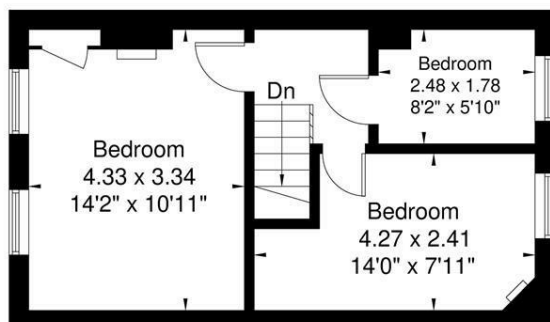
First Floor 33.9 sq m / 364 sq ft
