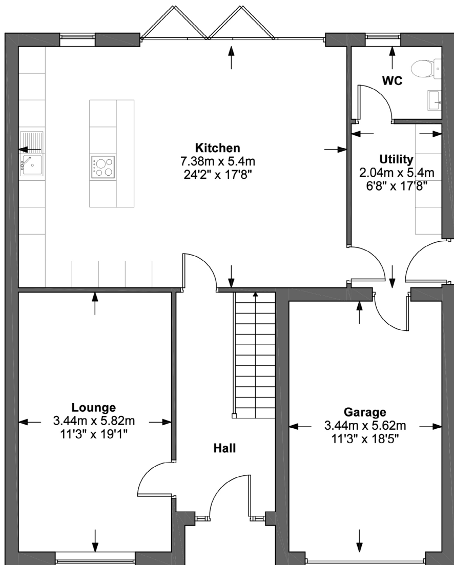
Elm Ground Floor Plan
