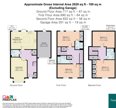
Floor Plan
