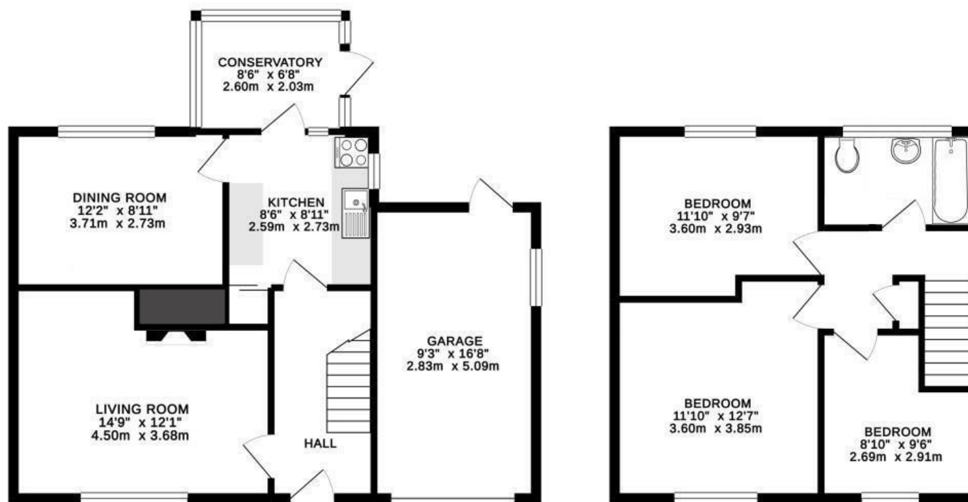
GROUND FLOOR
