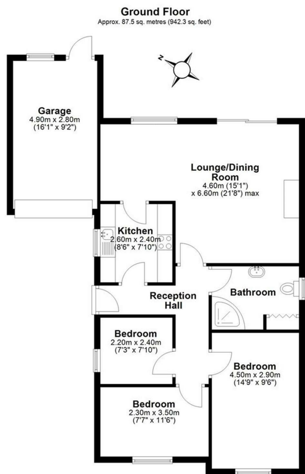
Total area: approx. 87.5 sq. metres (942.3 sq. feet) 59 Hollies Road
