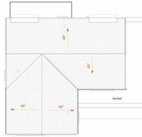
4 GA_Plan_Roof 1:100
