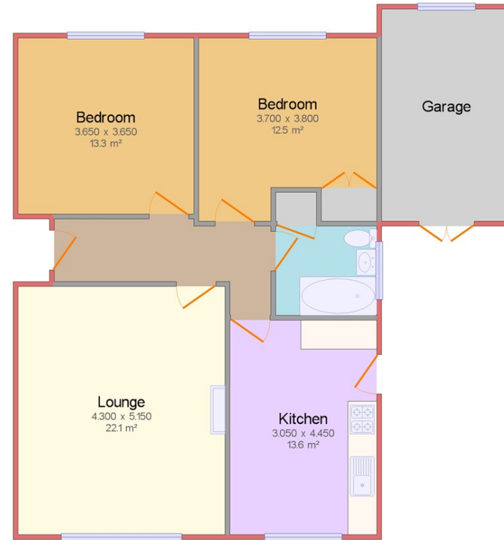
141 Gordon Field, Market Rasen - Floor Plan Gross internal area: 88.1 m 2 (948.0 ft 2 )
