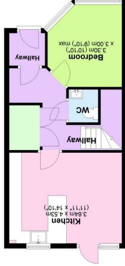
Ground Floor Approx. 41.0 sq. metres (441.4 sq. feet)
