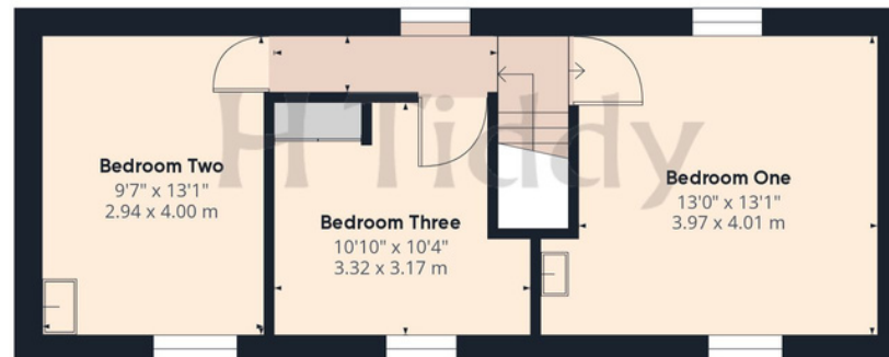
Floor 1 Building 1
