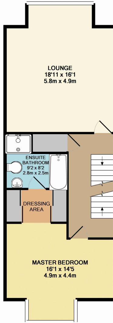
1ST FLOOR APPROX. FLOOR AREA 697 SQ.FT. (64.7 SQ.M.)
