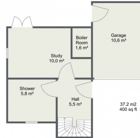
11 Brickfields Ground Floor
