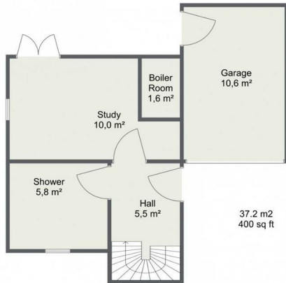
11 Brickfields Ground Floor
