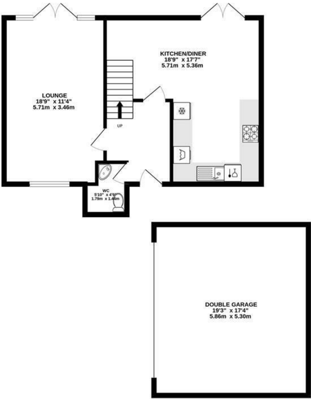
GROUND FLOOR 892 sq.ft. (82.8 sq.m.) approx.
