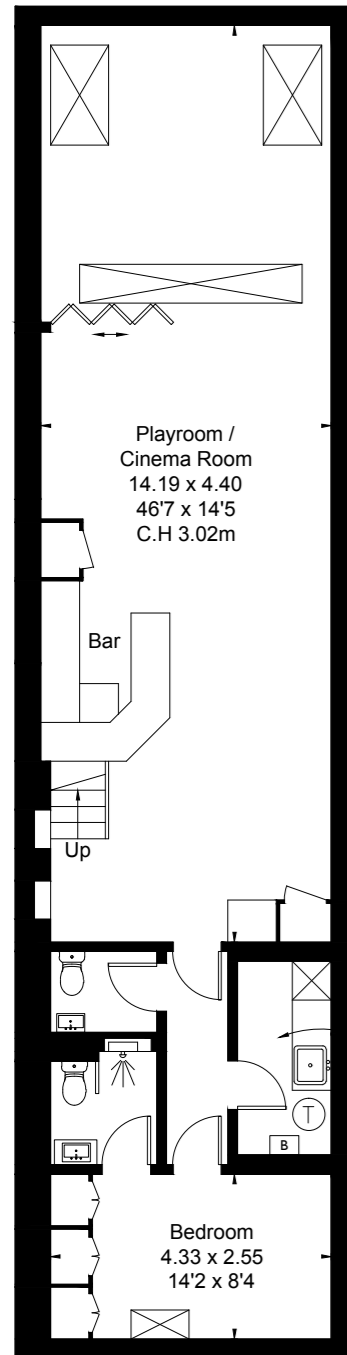
BASEMENT
