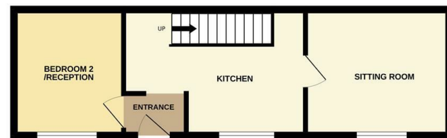
GROUND FLOOR 340 sq.ft. (31.5 sq.m.) approx.
