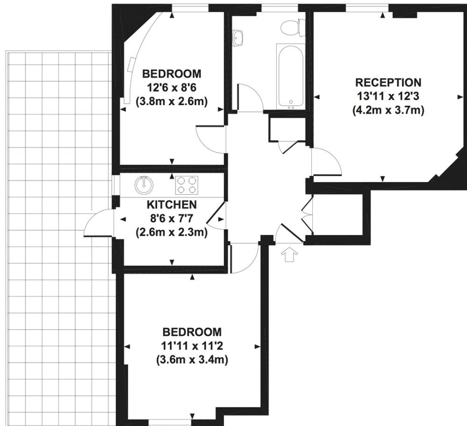
SECOND FLOOR
