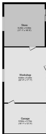
Outbuilding Floor area 81.5 m 2 (877 sq.ft.)
