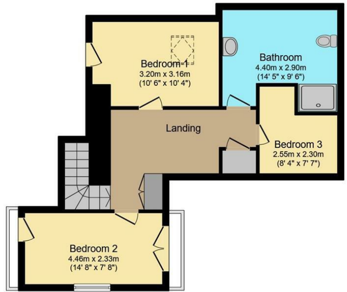
First Floor Floor area 58.9 m 2 (634 sq.ft.)
