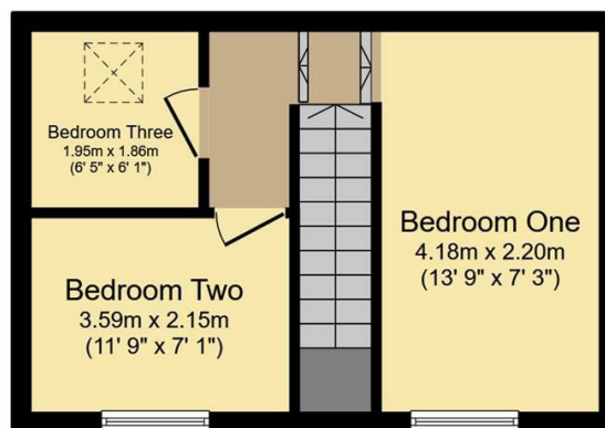
First Floor Floor area 26.3 m 2 (283 sq.ft.)
