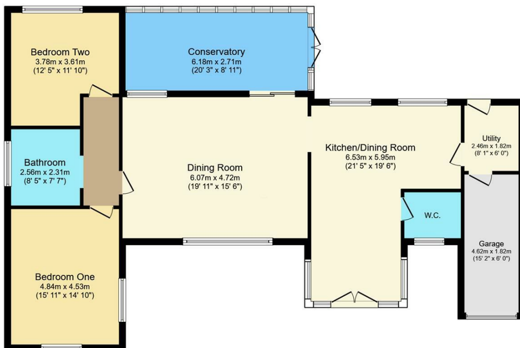
Floor Plan Floor area 129.2 m 2 (1,390 sq.ft.)
